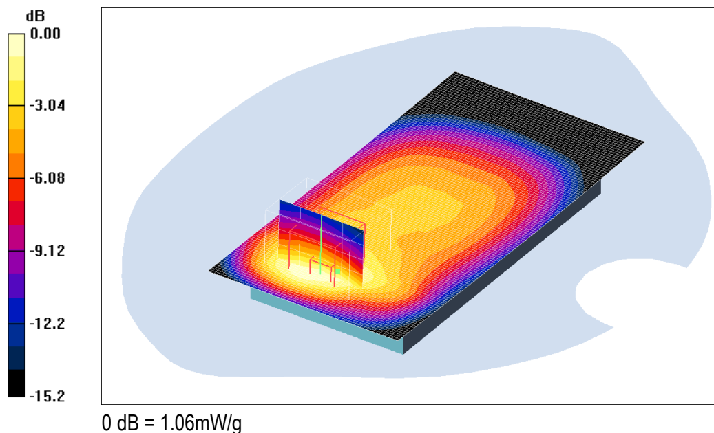
Fig. 10: canal 2863 (912.6 MHz) – face arrière - 5mm
