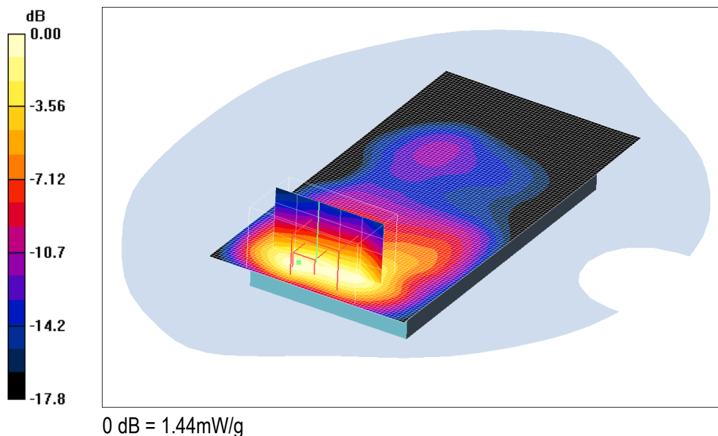
Fig. 13: canal 19575 (1747.5 MHz) – face arrière - 5mm
