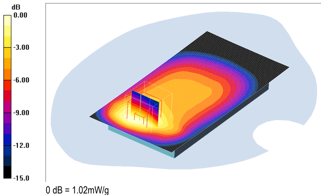
Fig. 8: canal 124 (914.8 MHz) – face arrière - 5mm
