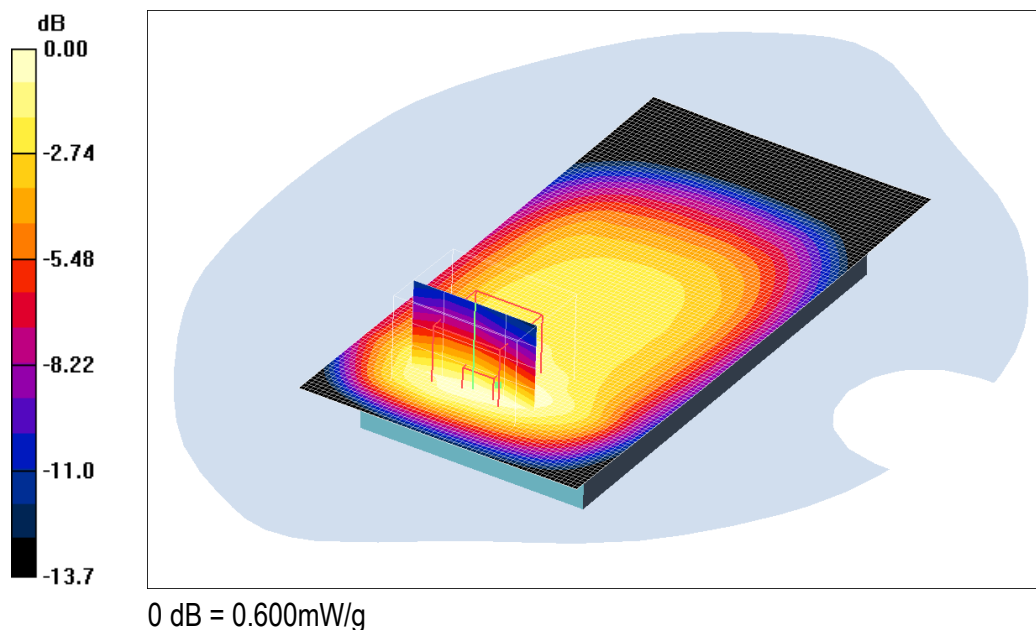
Fig. 12: canal 24300 (847.0 MHz) – face arrière - 5mm
