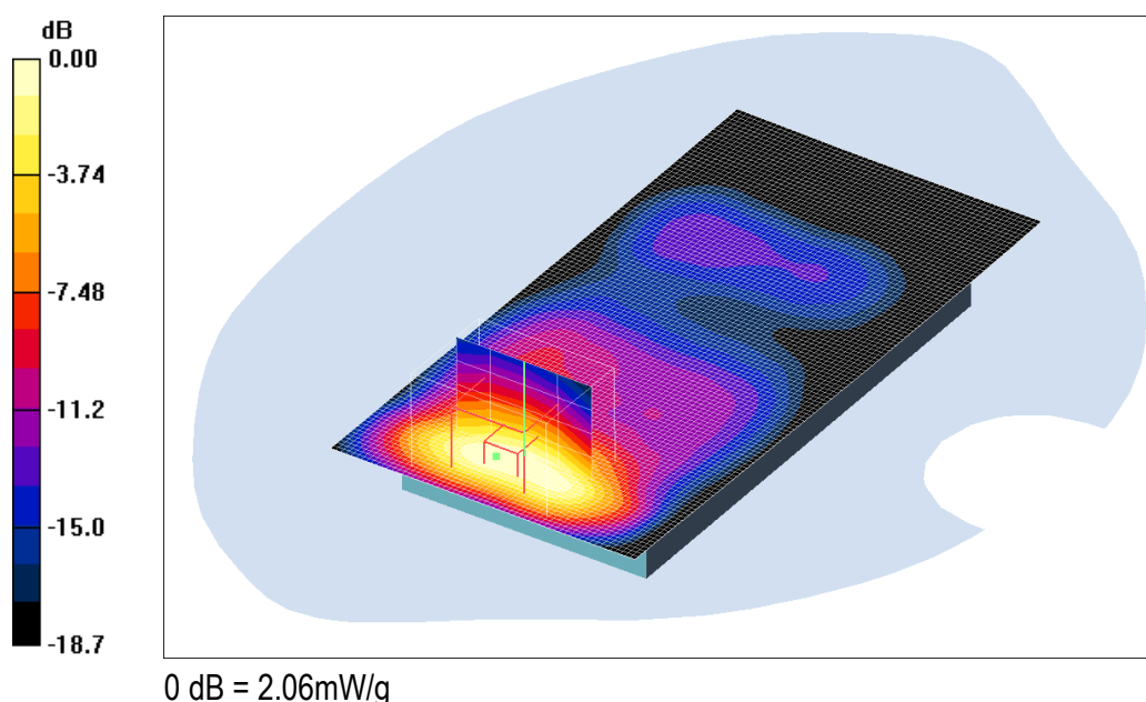
Fig. 11: canal 9888 (1977.6 MHz) – face arrière - 5mm
