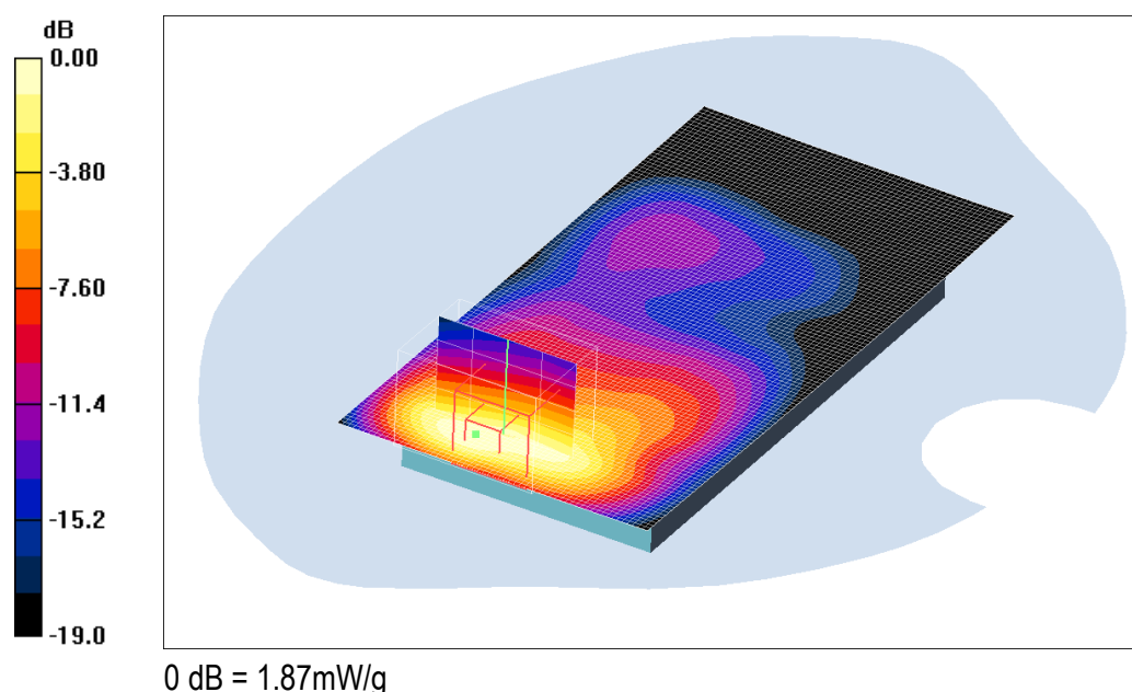
Fig. 9: canal 699 (1747.6 MHz) – face arrière - 5mm
