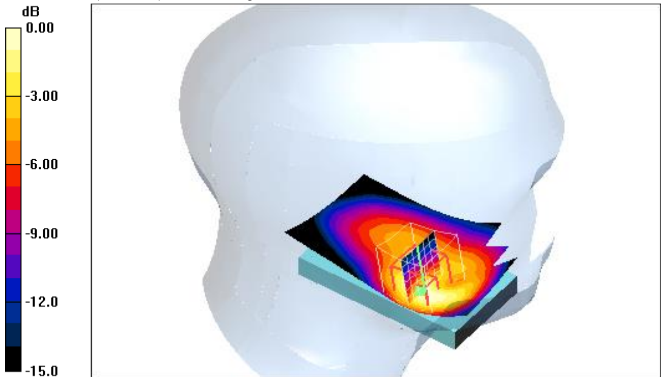
0 dB = 0.865mW/g
