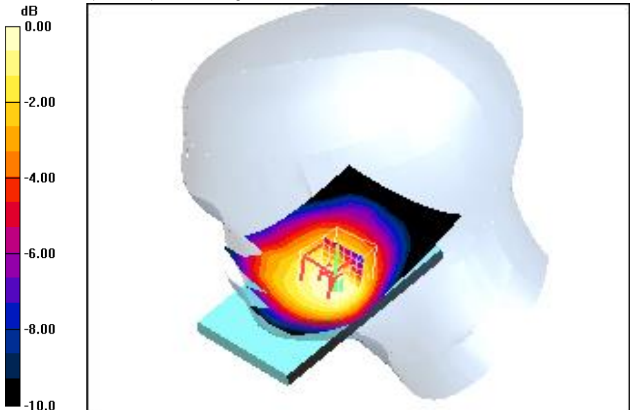
0 dB = 0.425mW/g
